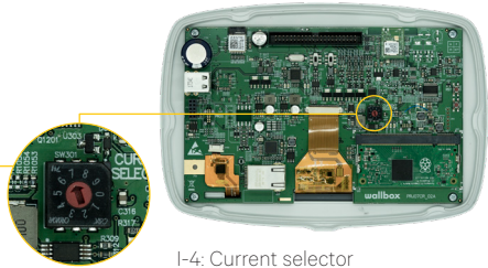
I-4: Current selector
