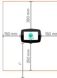
I-2.1: Monteringsyta
