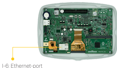
I-6: Ethernet-port
